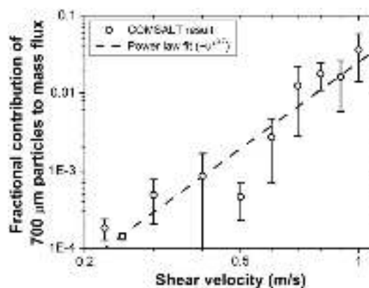
Fig. 18. The fractional contribution of 700\ \mu\text{m} particles to the streamwise mass flux over a soil bed with equal surface fractions of 180 and 700\ \mu\text{m} particles, simulated with the numerical saltation model COMSALT (Kok and Renno, 2009a). Each data point denotes the average and standard error of eight separate simulations that generated varying results because of the stochastic nature of COMSALT (Kok and Renno, 2009a). The dashed line denotes a least squares power law fit to the simulation results.
