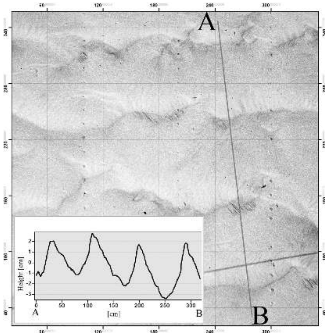
Fig. 3. Typical megaripples at Nahal Kasuy (the square grid is 60 × 60 cm). The inset shows the photogrammetry profile along a cross-section (line AB). The average wavelength was 70 cm and the average height was about 4 cm (the wind direction was from B to A).
