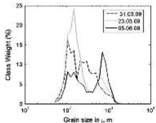
Fig. 13. Grain size analyses of crest samples taken before the storms (05.06.08), after the first storm (23rd March 2009) and after the second storm (31st March 2009). The typical bimodal distribution of megaripples changed to a unimodal distribution of normal ripples.
