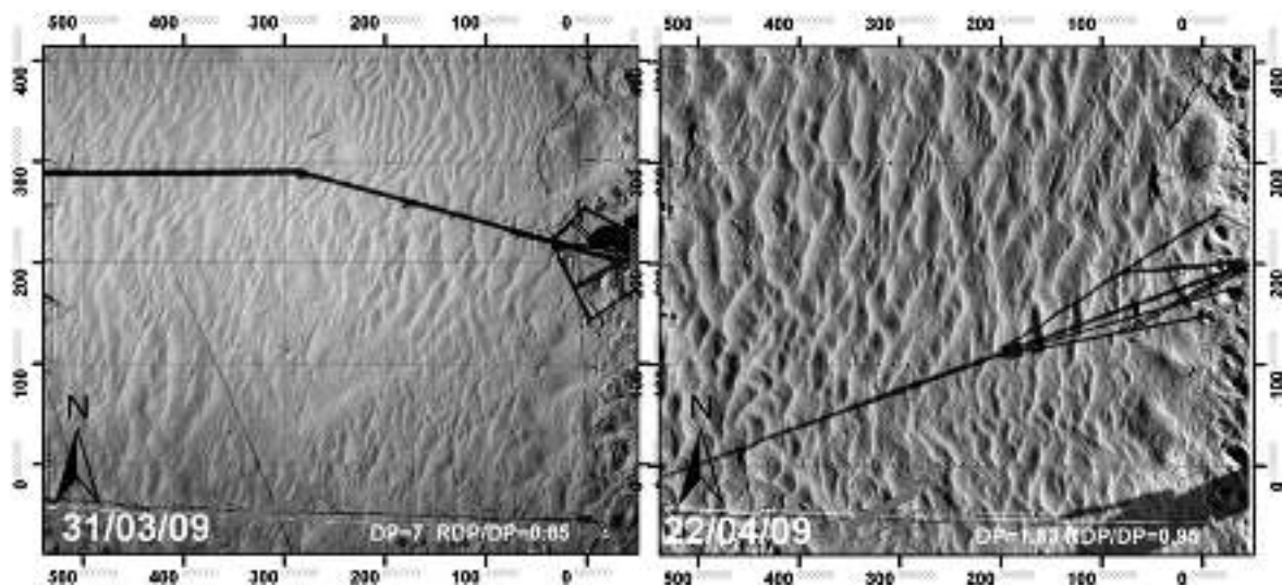
Fig. 17. Initial development of normal ripples in Plot D after megariipple destruction on 31st March 2009. The red arrows show the direction of RDP during the period between the previous and the current visits.
