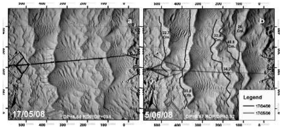
Fig. 16. Plot D before and after the storm of 8th May 2008. Panel (a) shows the location of megariipple crest-lines on 17th May. Panel (b) shows the crest lines both of 17th April and of 17th May. Note that there was almost no change during the period from 17th May to 5th June 2008 as DP was very low. The numbers between the two crest lines (panel b) indicate the average distance the megaripples moved downwind (the grid is 1 × 1 m).
