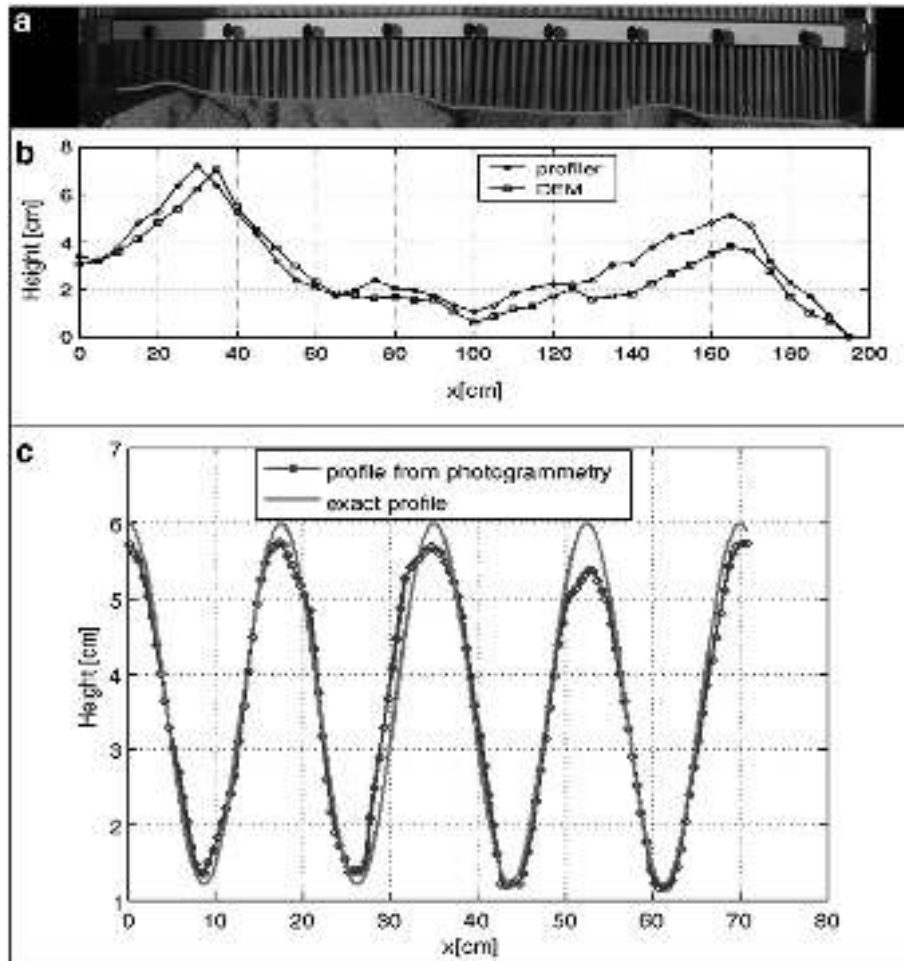
Fig. 5. (a) The profler used to measure megarripple profiles in plot E. (b) The measured and DEM profiles are shown together. (The wind direction is from left to right.) The agreement between the two is highly satisfactory (the average error was about 2%). (c) Validation using a piece of asbestos with a wavy surface. Also in this case there was good agreement between the DEM method and direct measurement (the average error was about 1%).
